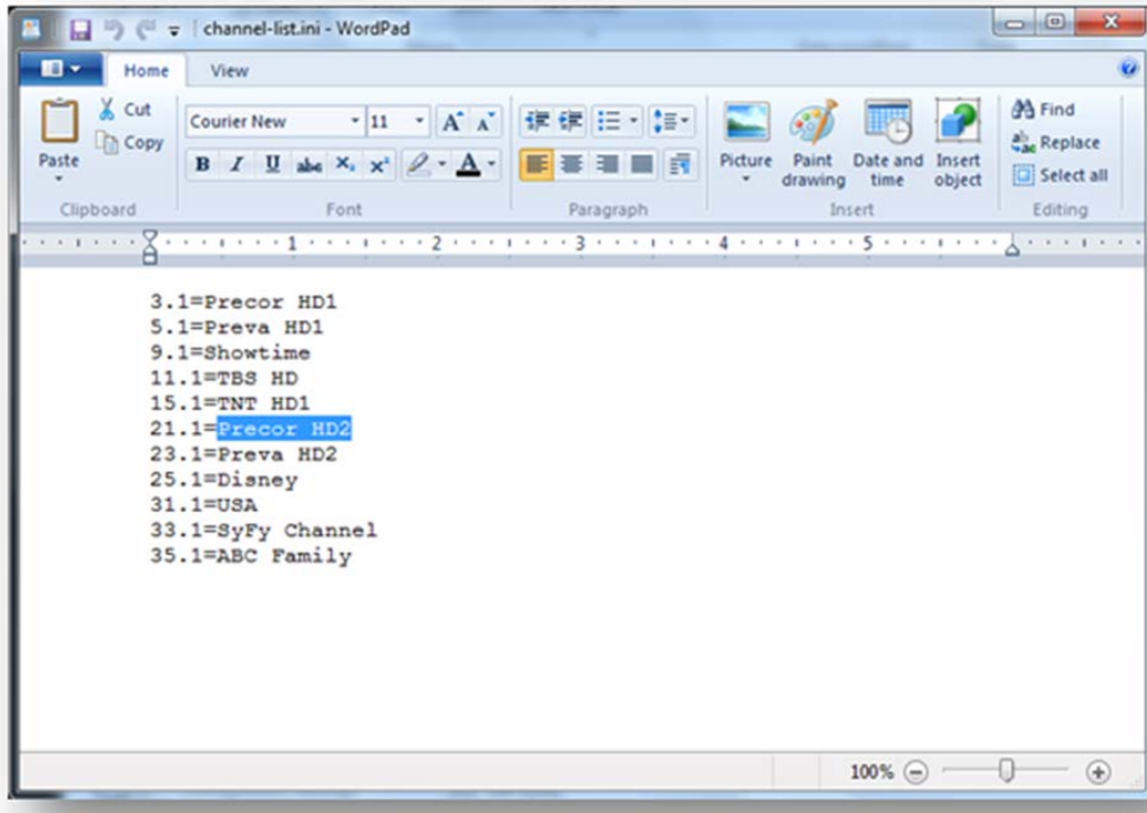
Figure 45: WordPad List
