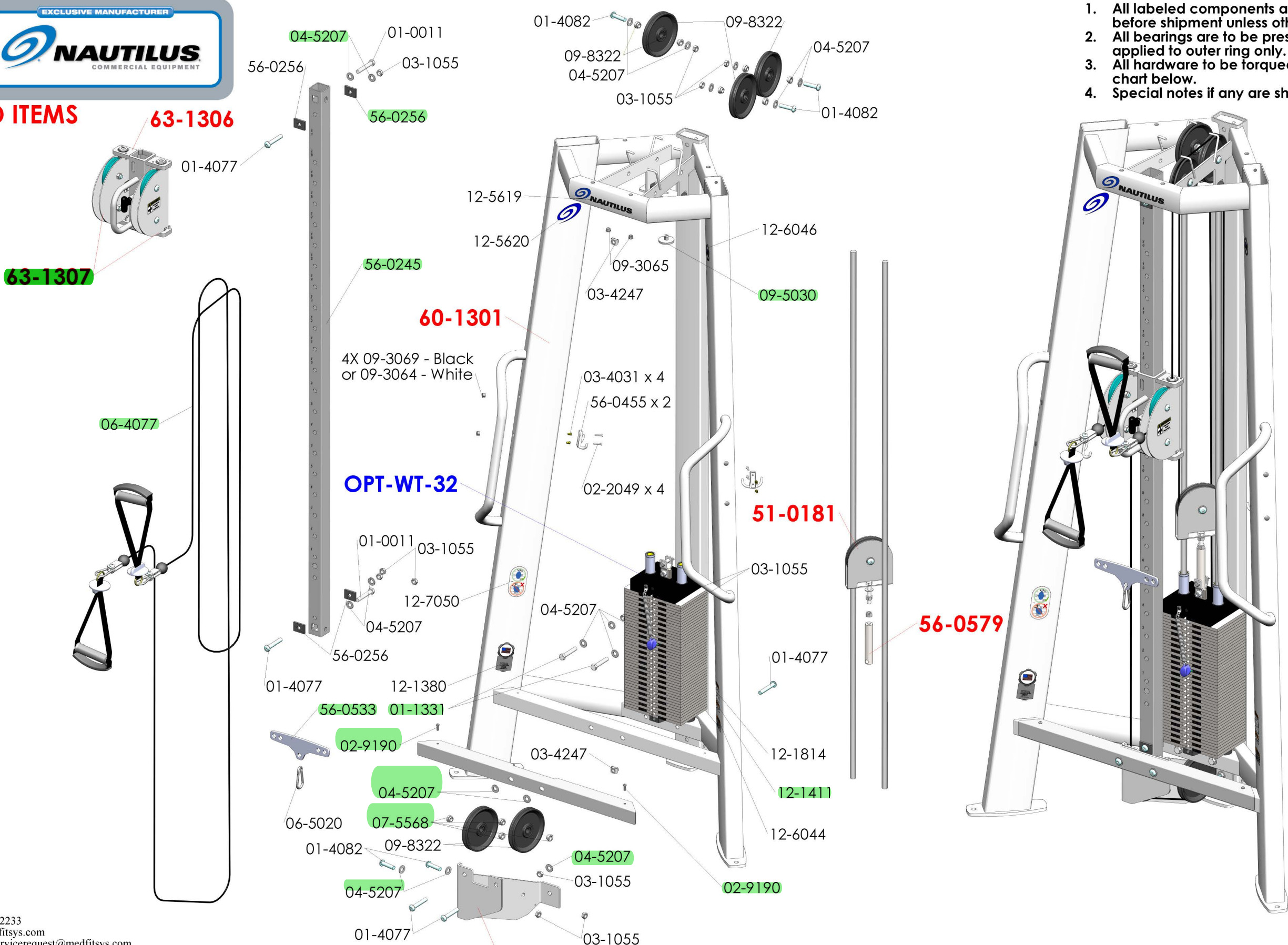
F3 Adjustable Tower (With EVO Medical Weight Stack) F3AT-M
