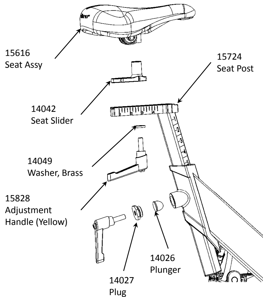
Seat Exploded View
